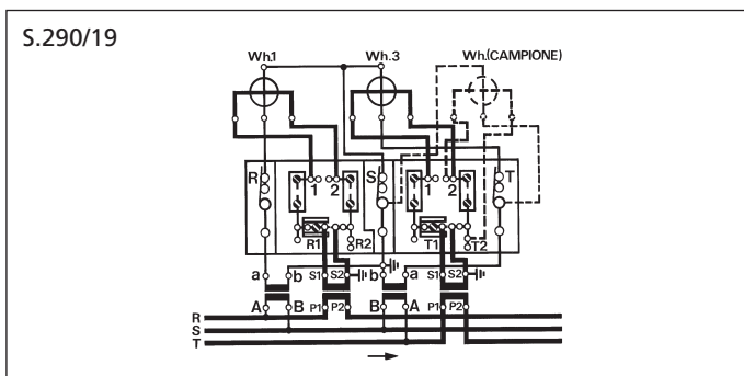
3-phase 2 systems KWh-meters
