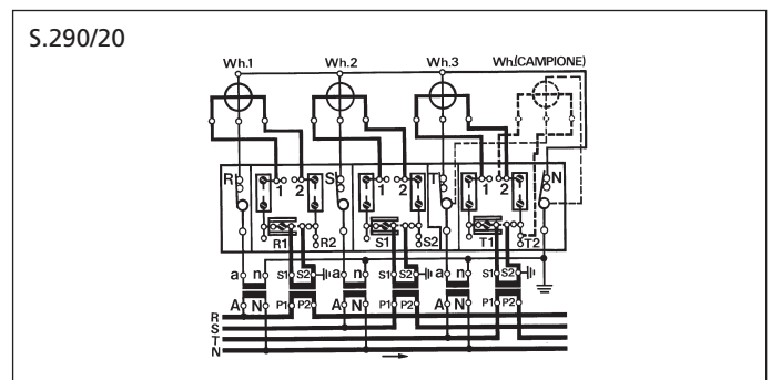
3-phase 3 systems KWh-meters
